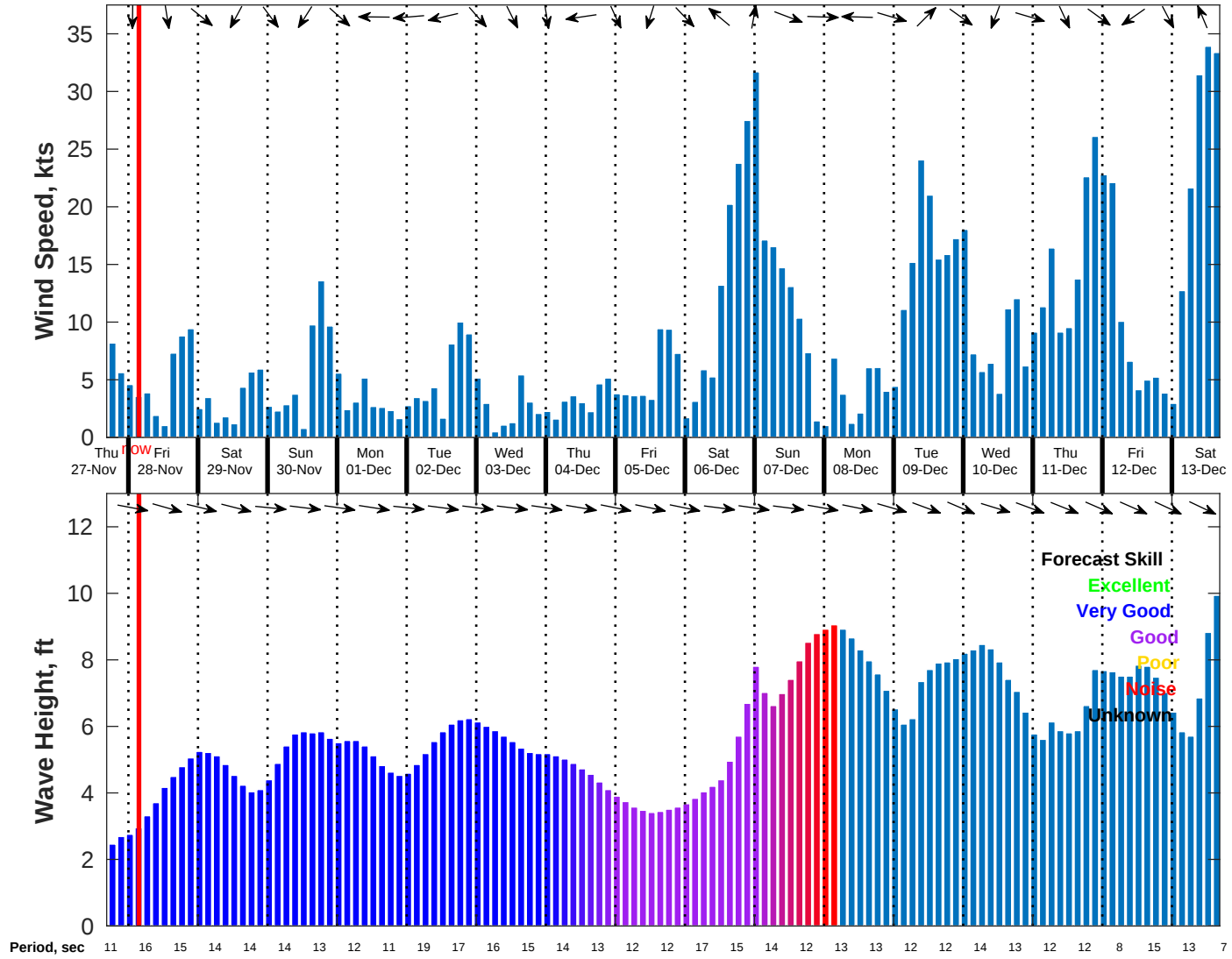
Wind & Wave Forecast for Diablo Canyon CDIP GFS from 27-Nov-2025 17:00:00 to 13-Dec-2025 17:00:00
