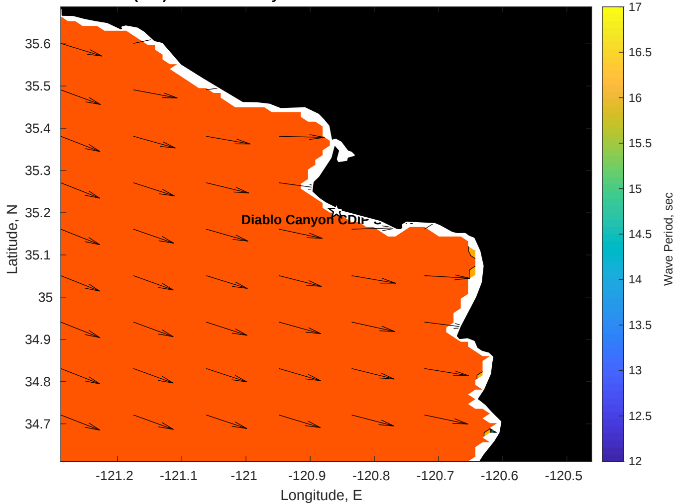
SWAN Wave Period (sec) for Diablo Canyon CDIP SWAN at 28-Nov-2025 10:00:00
