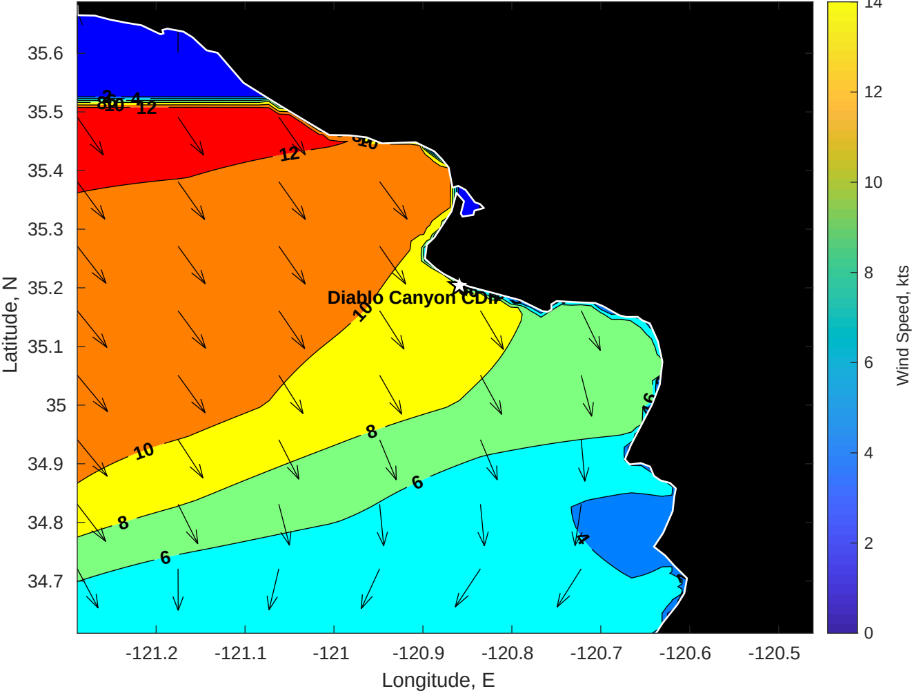
SWAN Winds (kts) for Diablo Canyon CDIP SWAN at 28-Nov-2025 10:00:00
