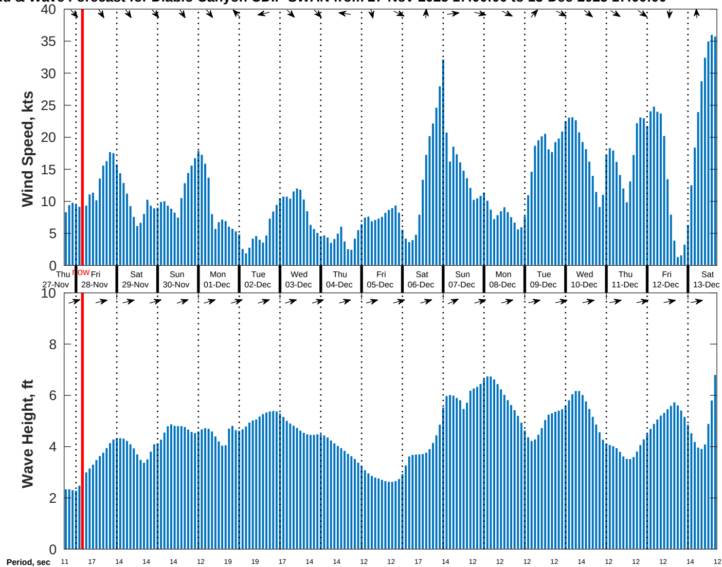
Wind & Wave Forecast for Diablo Canyon CDIP SWAN from 27-Nov-2025 17:00:00 to 13-Dec-2025 17:00:00
