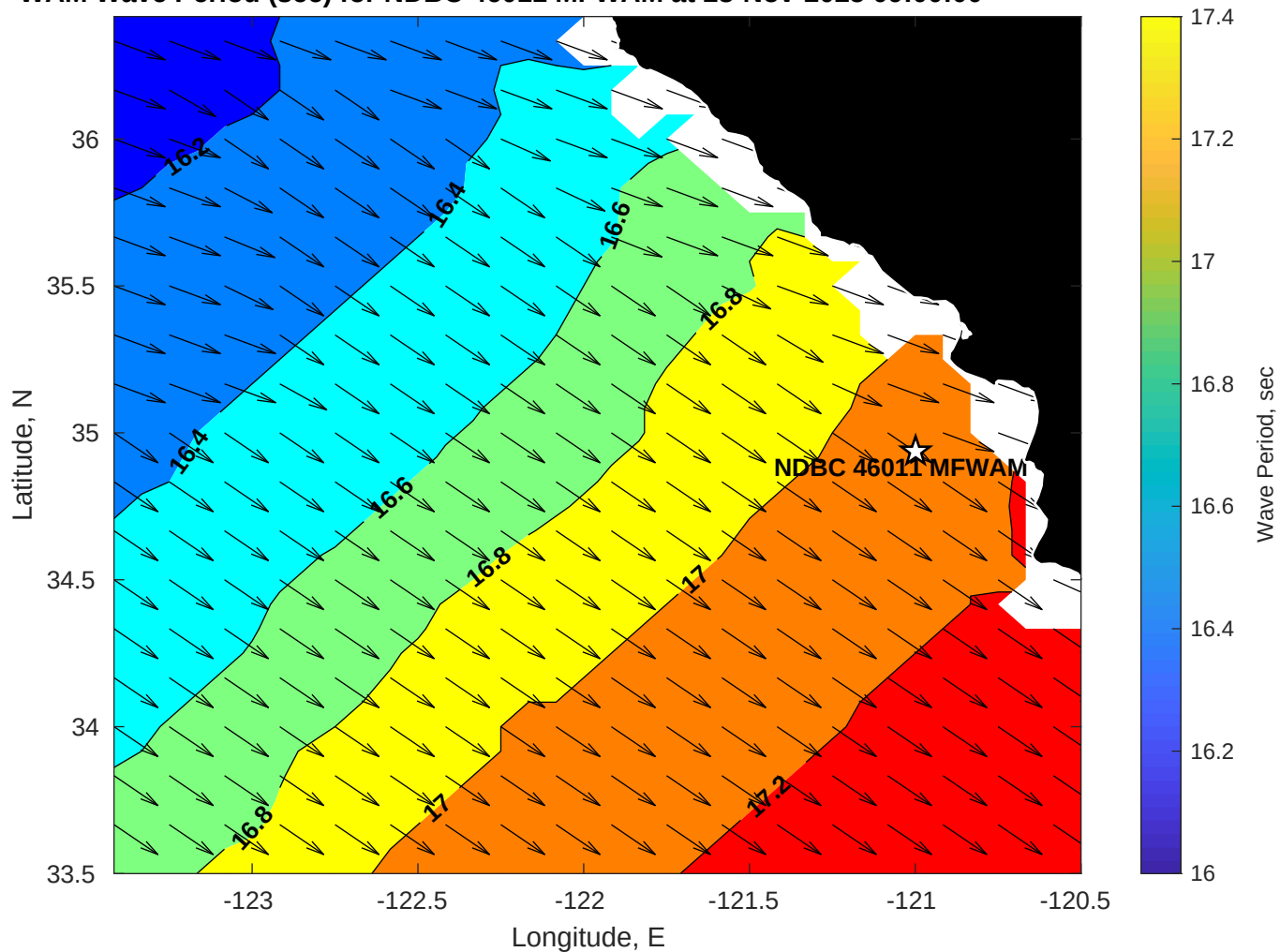
WAM Wave Period (sec) for NDBC 46011 MFWAM at 28-Nov-2025 09:00:00
