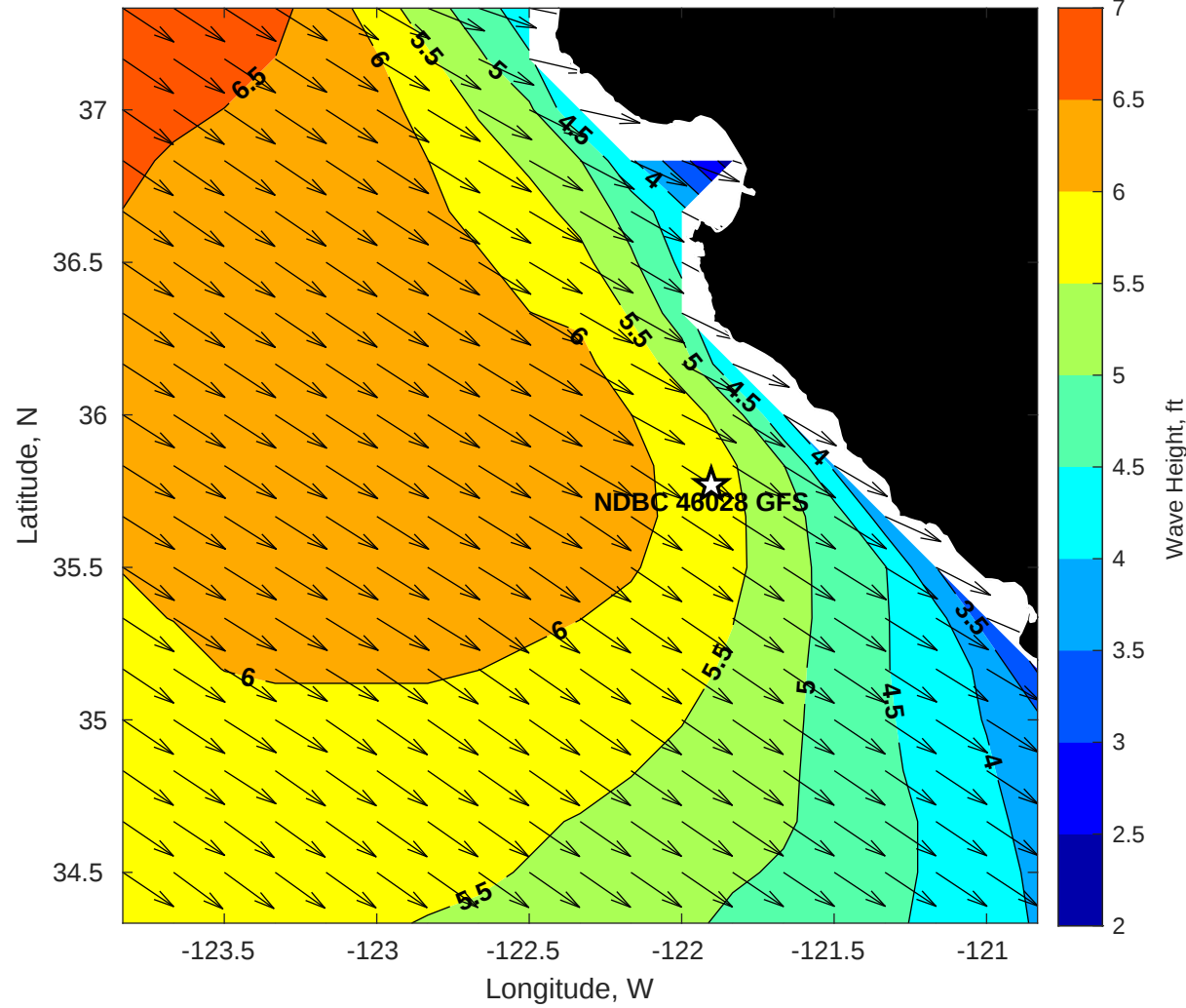
GFS Wave Height (ft) for NDBC 46028 GFS at 28-Nov-2025 09:00:00
