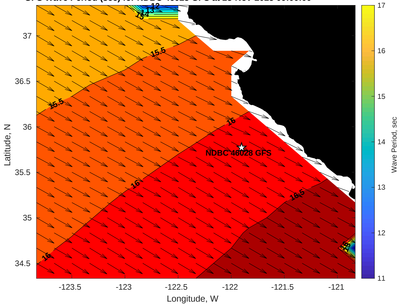
GFS Wave Period (sec) for NDBC 46028 GFS at 28-Nov-2025 09:00:00
