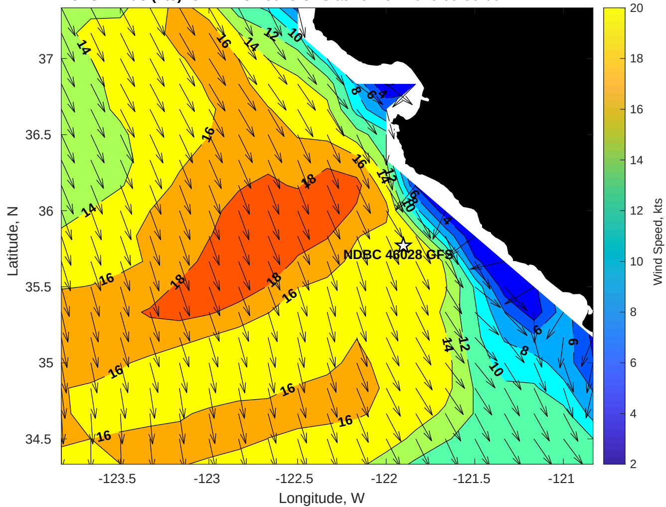
GFS Winds (kts) for NDBC 46028 GFS at 28-Nov-2025 09:00:00
