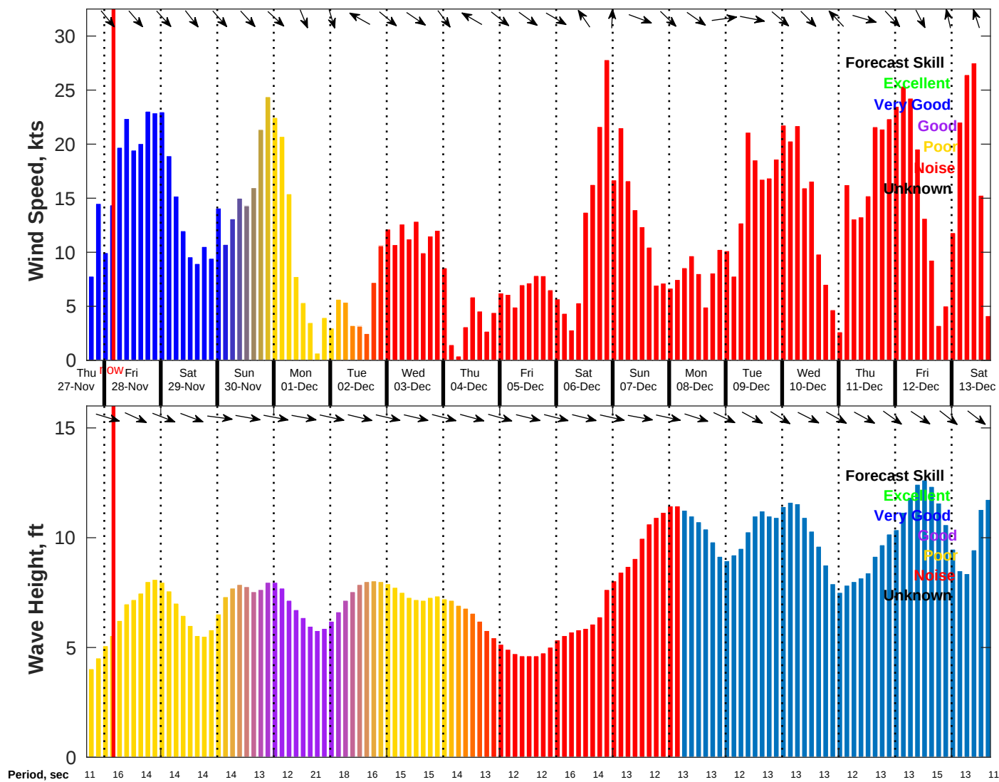
Wind & Wave Forecast for NDBC 46028 GFS from 27-Nov-2025 17:00:00 to 13-Dec-2025 17:00:00
