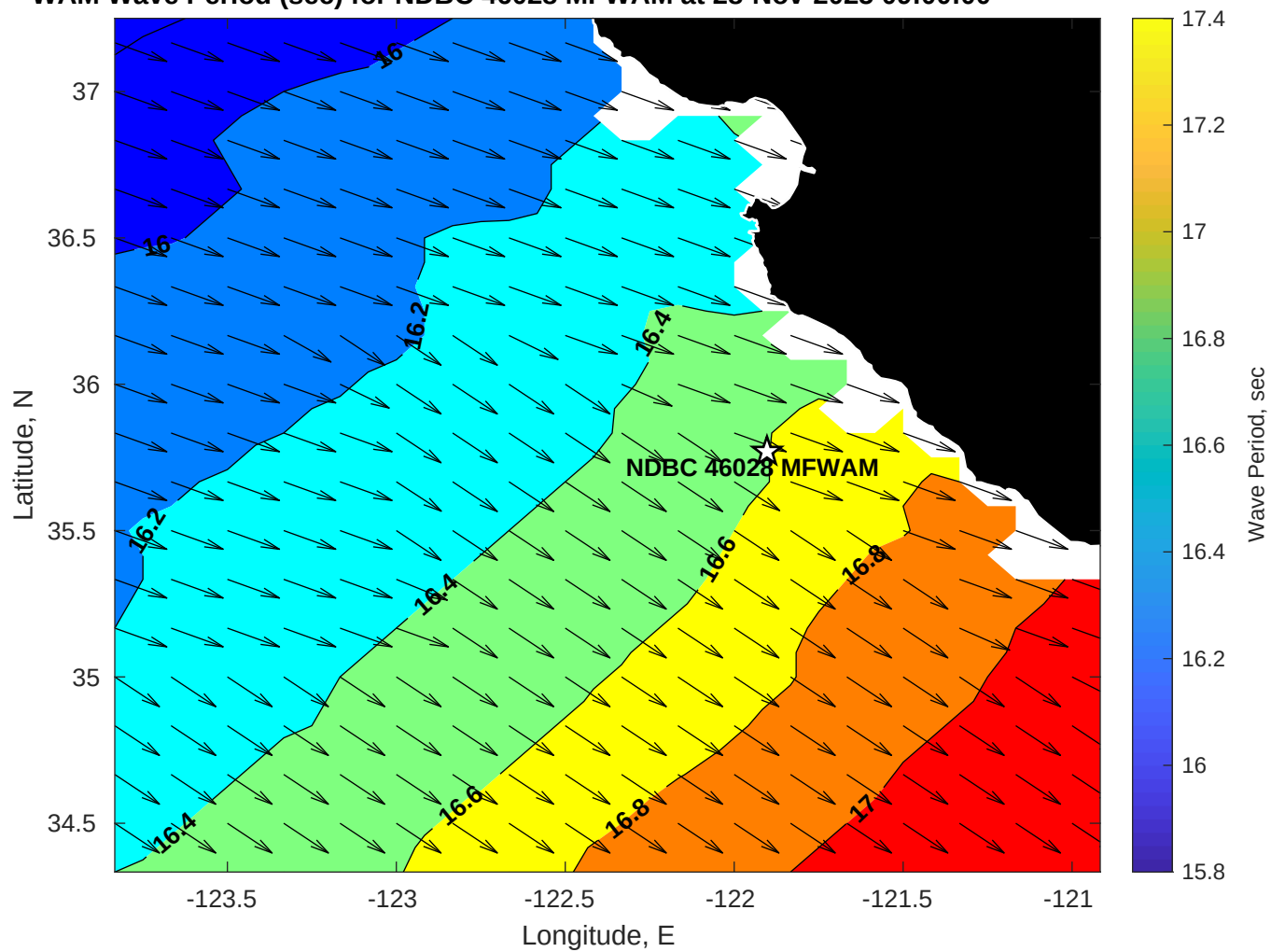
WAM Wave Period (sec) for NDBC 46028 MFWAM at 28-Nov-2025 09:00:00
