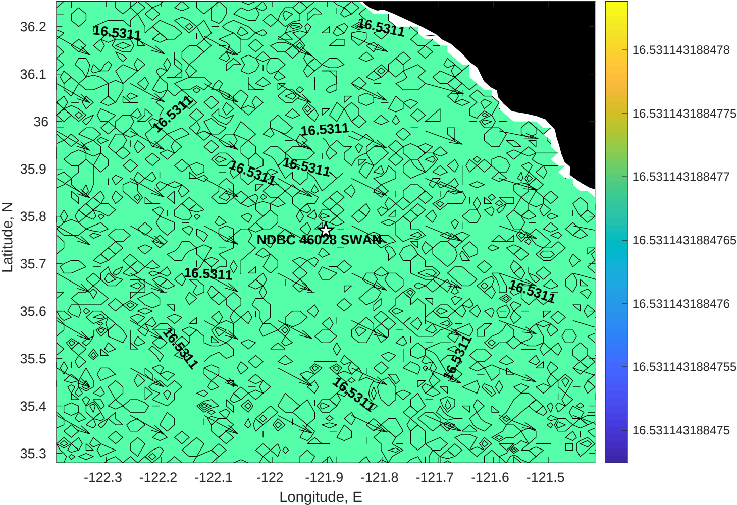
SWAN Wave Period (sec) for NDBC 46028 SWAN at 28-Nov-2025 10:00:00
