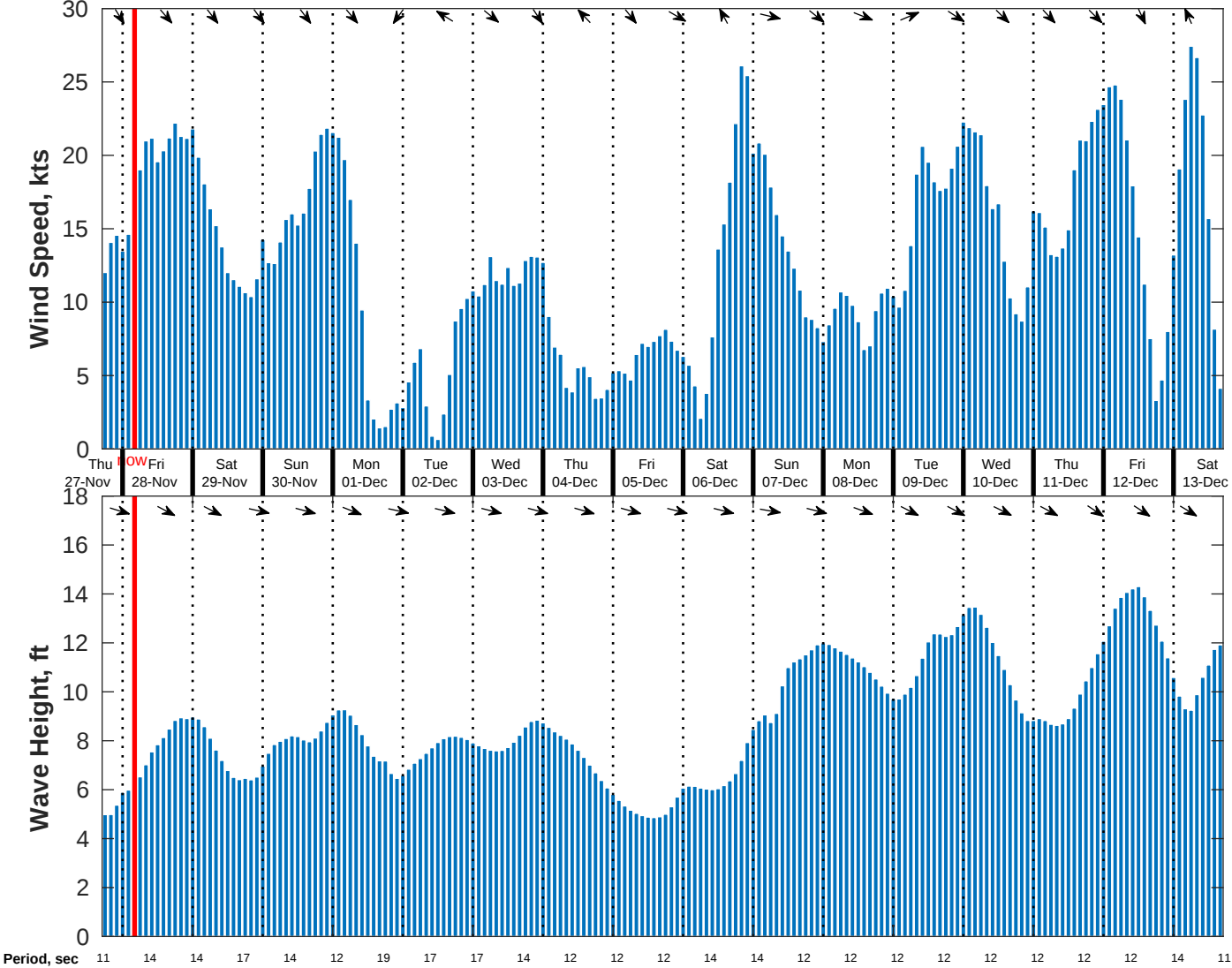
Wind & Wave Forecast for NDBC 46028 SWAN from 27-Nov-2025 17:00:00 to 13-Dec-2025 17:00:00
