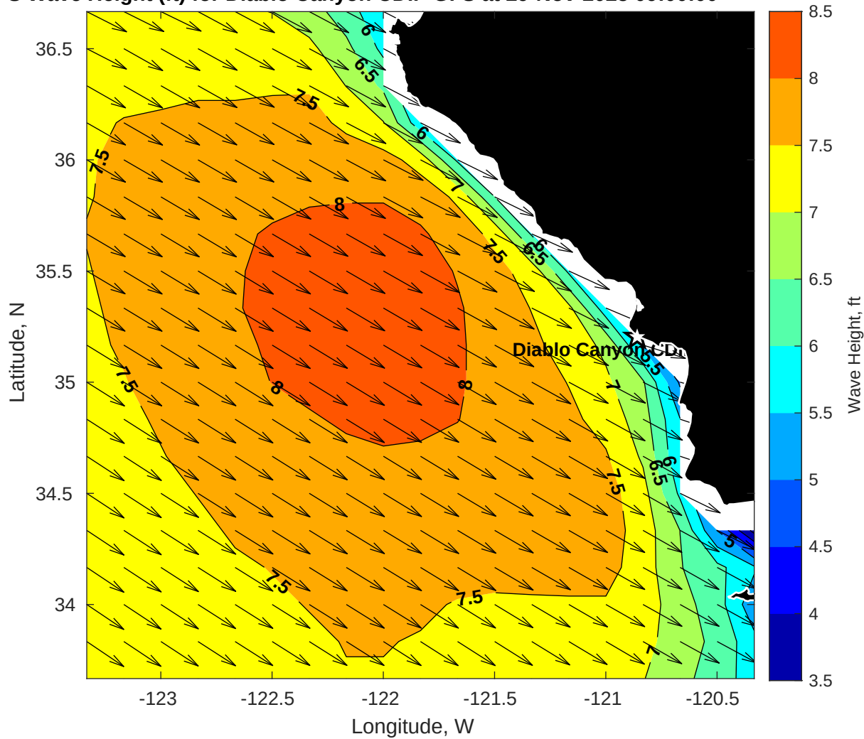
GFS Wave Height (ft) for Diablo Canyon CDIP GFS at 29-Nov-2025 09:00:00
