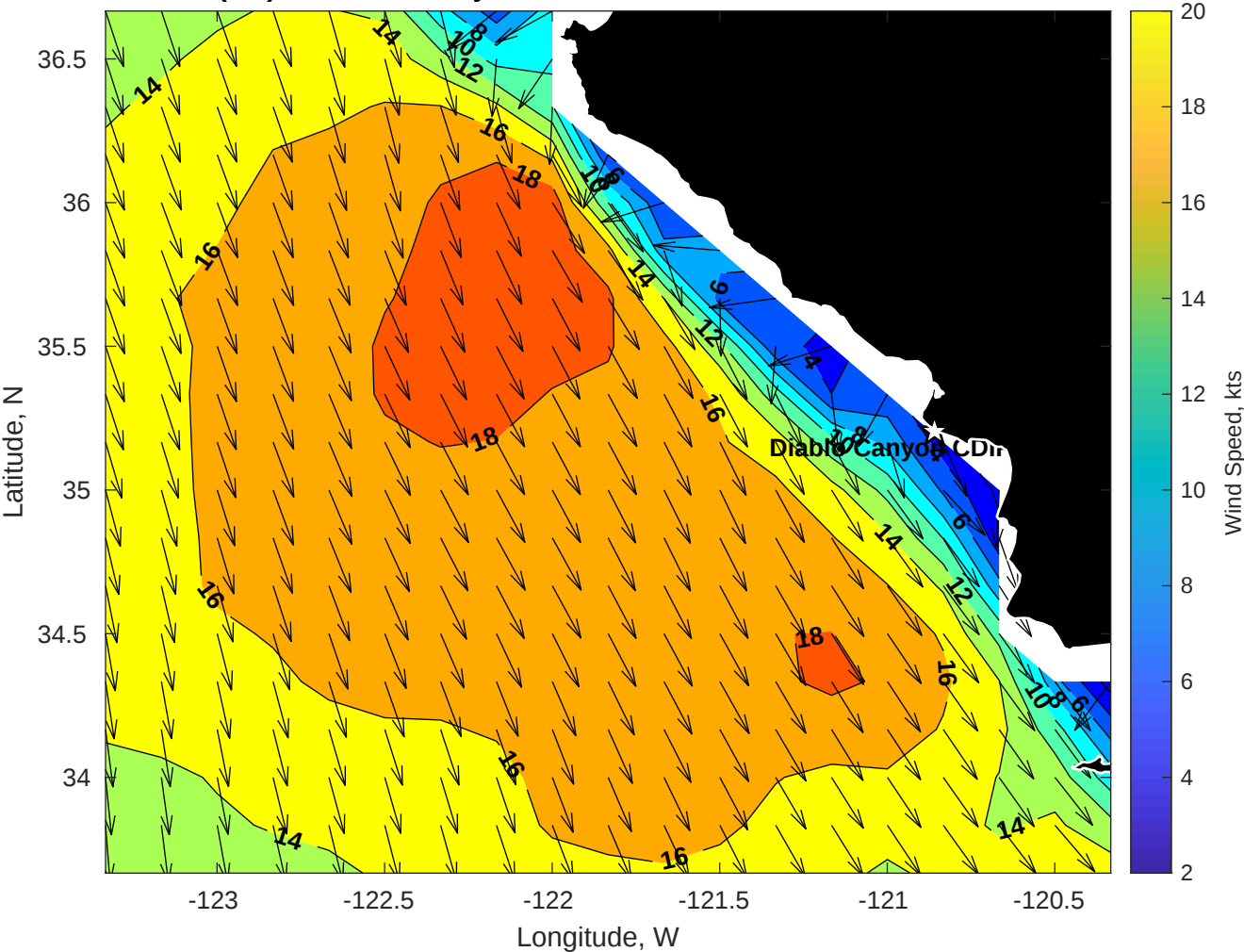
GFS Winds (kts) for Diablo Canyon CDIP GFS at 29-Nov-2025 09:00:00
