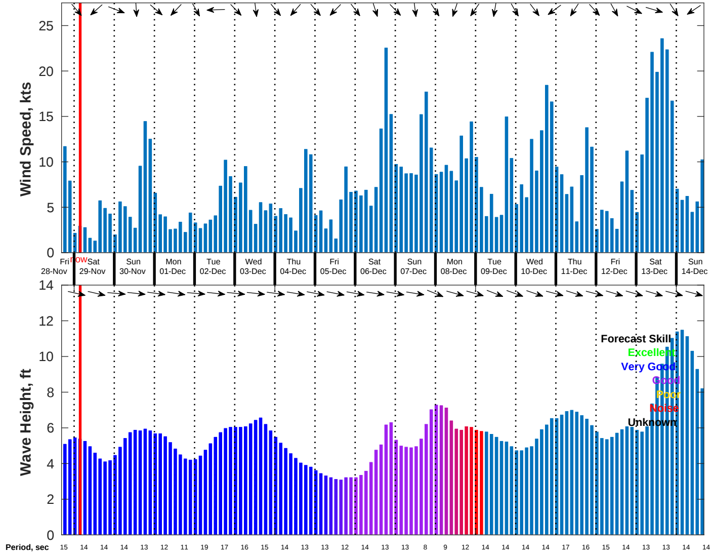
Wind & Wave Forecast for Diablo Canyon CDIP GFS from 28-Nov-2025 17:00:00 to 14-Dec-2025 17:00:00
