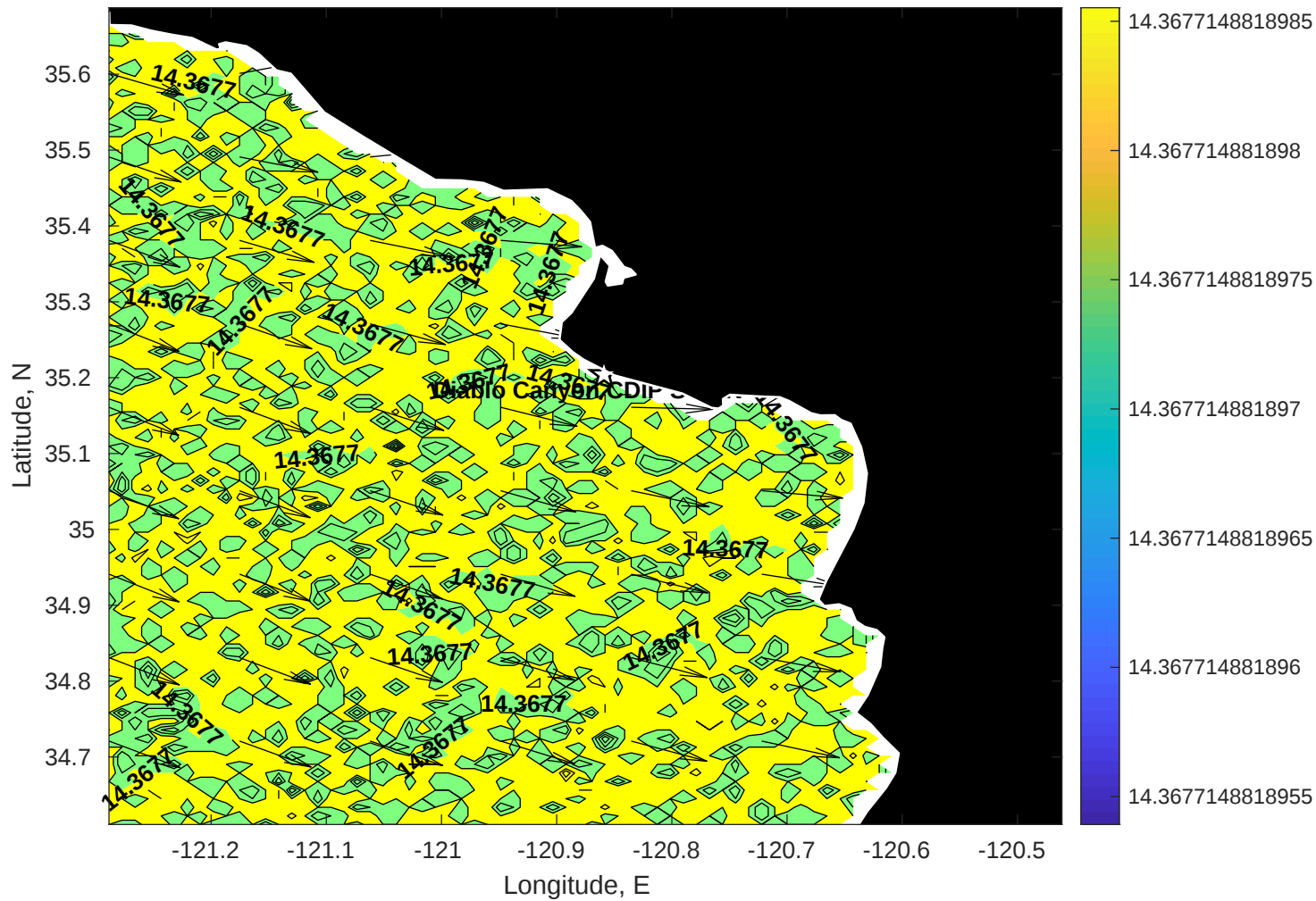
SWAN Wave Period (sec) for Diablo Canyon CDIP SWAN at 29-Nov-2025 10:00:00
