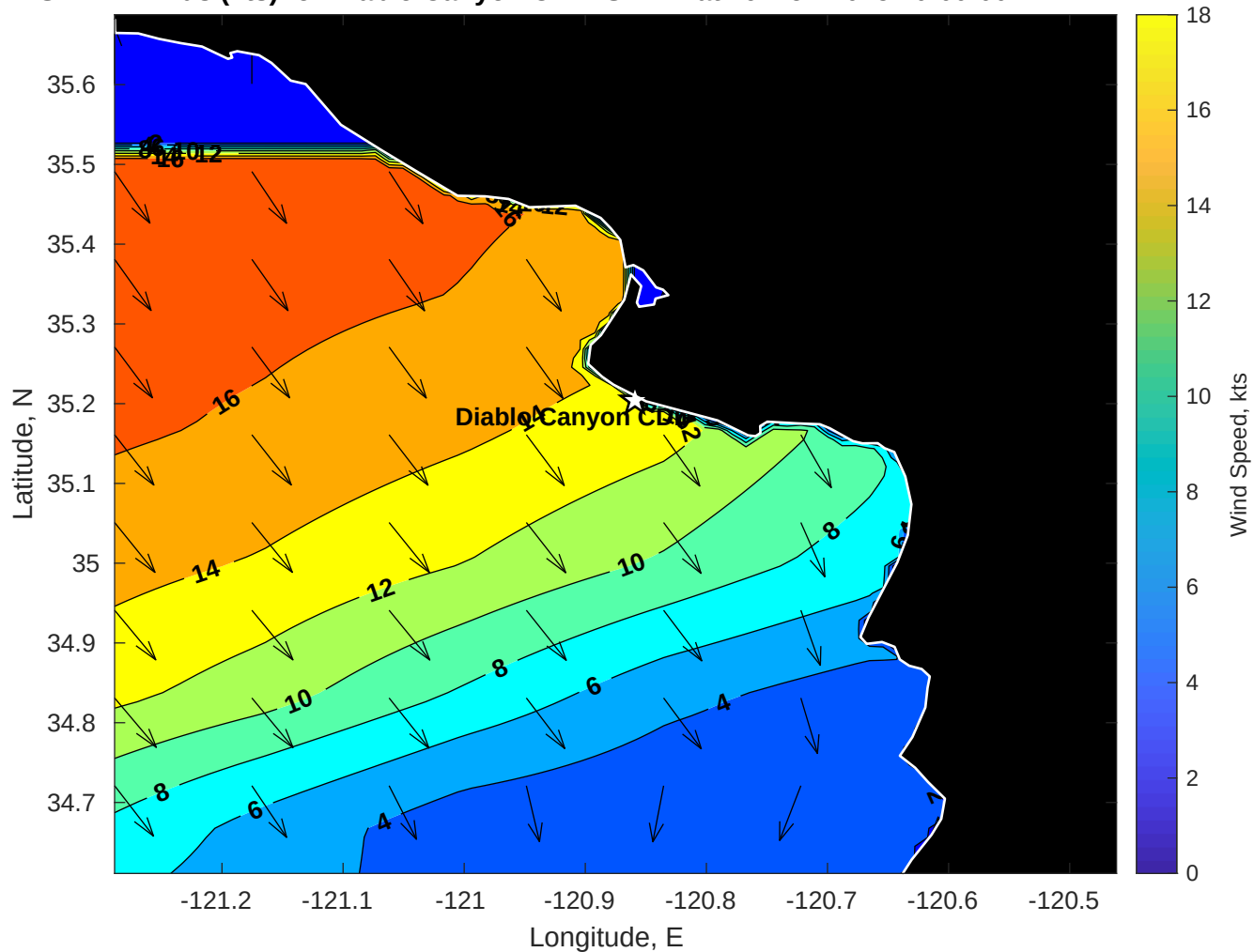
SWAN Winds (kts) for Diablo Canyon CDIP SWAN at 29-Nov-2025 10:00:00
