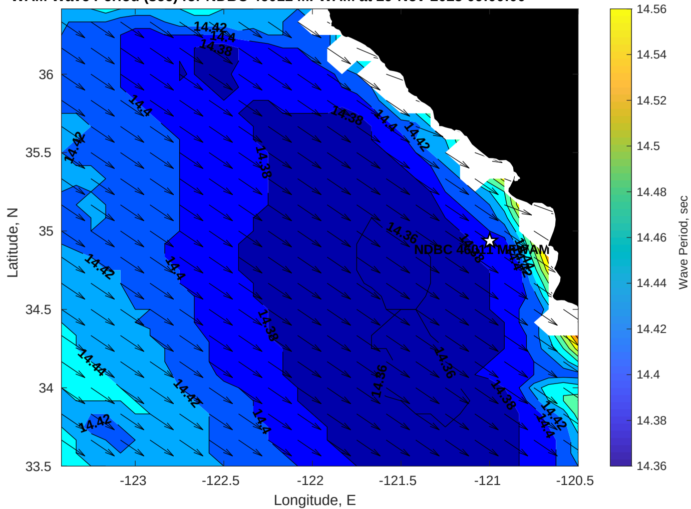
WAM Wave Period (sec) for NDBC 46011 MFWAM at 29-Nov-2025 09:00:00
