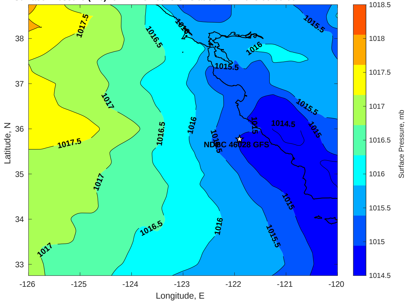
Surface Pressure (mb) for NDBC 46028 GFS at 30-Nov-2025 00:00:00
