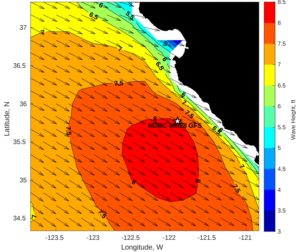
GFS Wave Height (ft) for NDBC 46028 GFS at 29-Nov-2025 09:00:00
