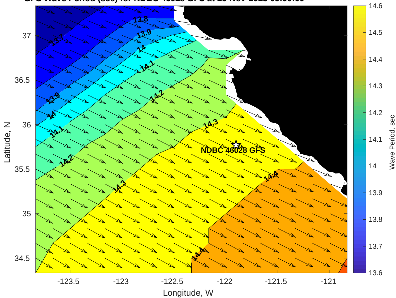
GFS Wave Period (sec) for NDBC 46028 GFS at 29-Nov-2025 09:00:00
