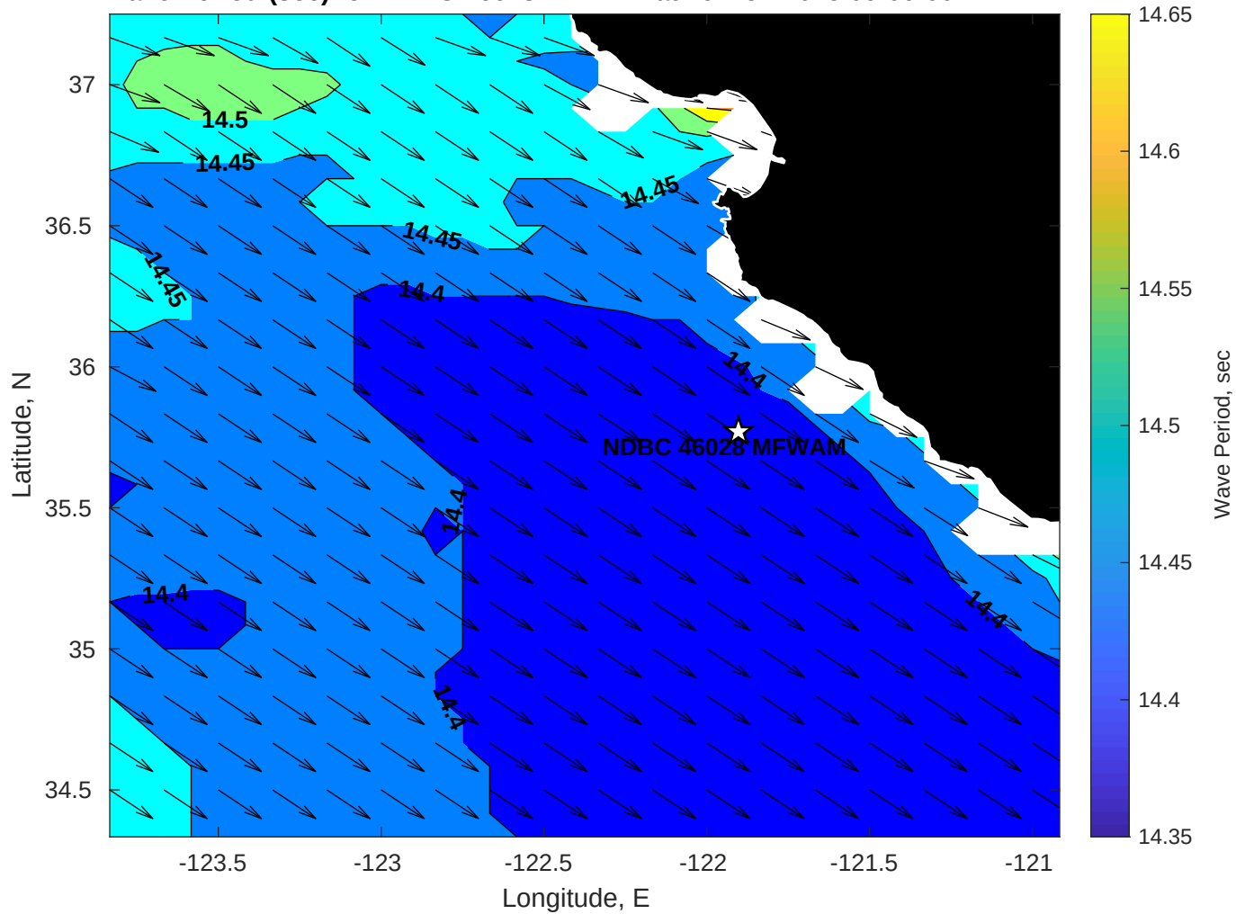
WAM Wave Period (sec) for NDBC 46028 MFWAM at 29-Nov-2025 09:00:00
