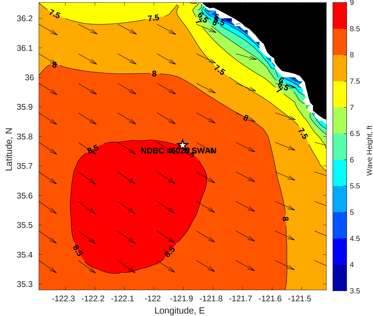
SWAN Wave Height (ft) for NDBC 46028 SWAN at 29-Nov-2025 10:00:00
