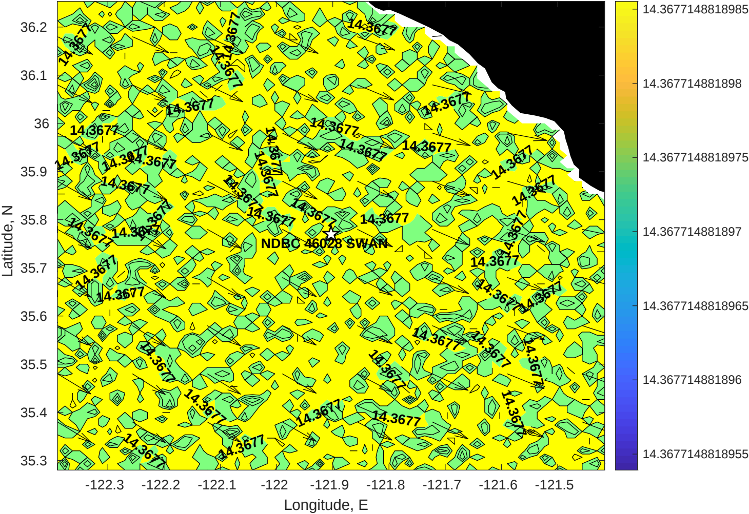
SWAN Wave Period (sec) for NDBC 46028 SWAN at 29-Nov-2025 10:00:00
