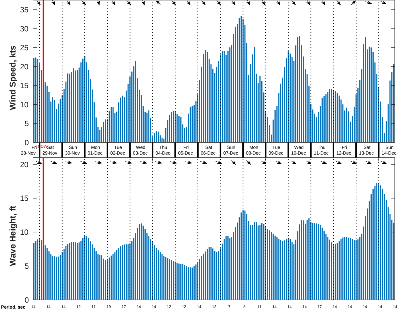
Wind & Wave Forecast for NDBC 46028 SWAN from 28-Nov-2025 17:00:00 to 14-Dec-2025 17:00:00
