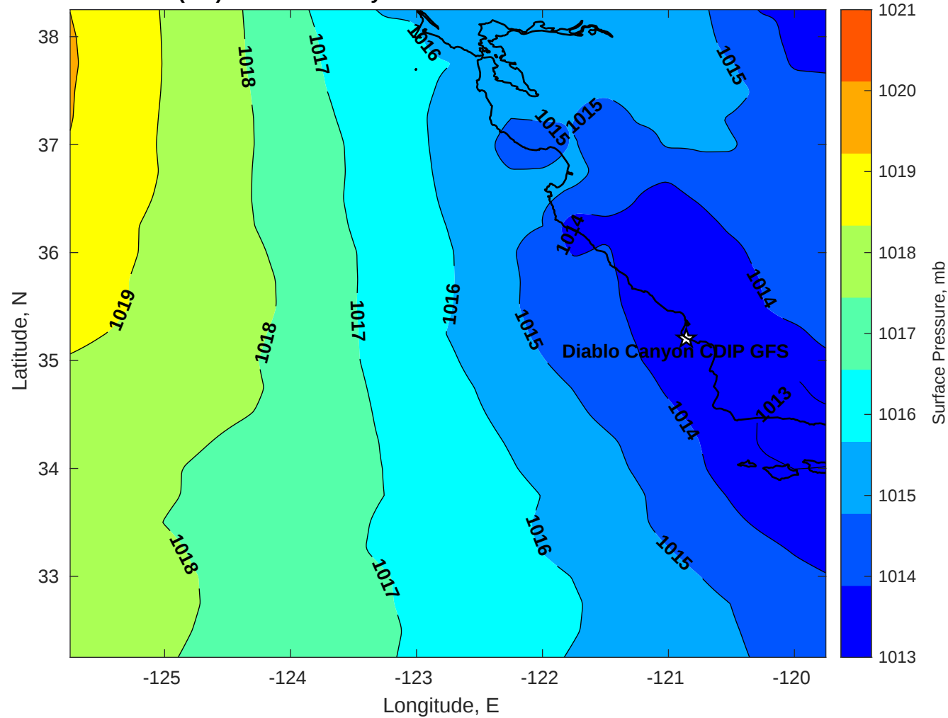
Surface Pressure (mb) for Diablo Canyon CDIP GFS at 01-Dec-2025 00:00:00
