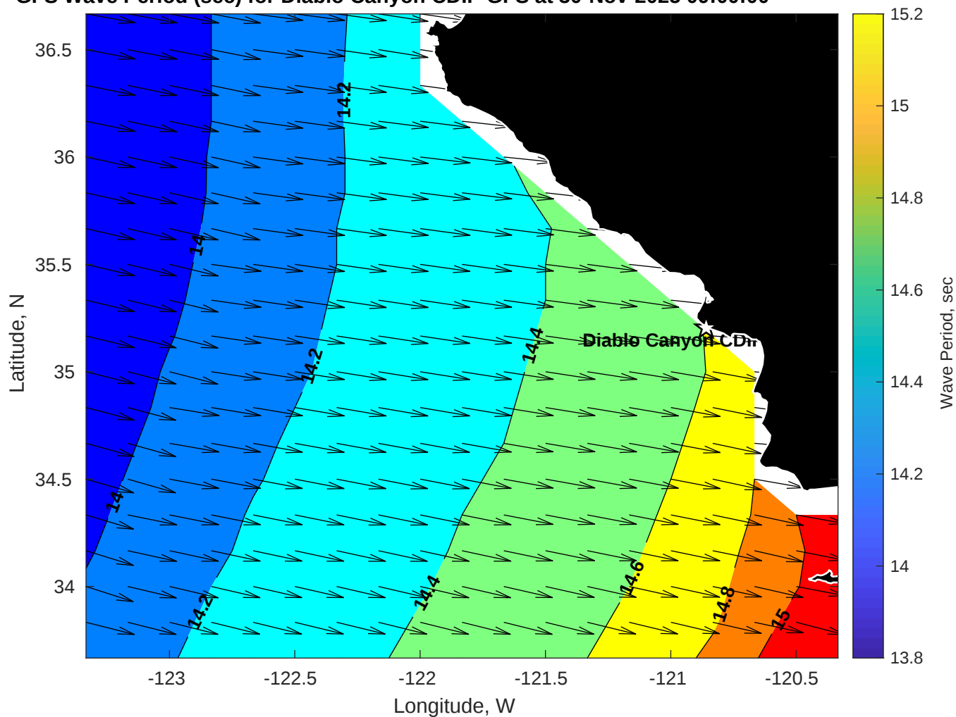
GFS Wave Period (sec) for Diablo Canyon CDIP GFS at 30-Nov-2025 09:00:00
