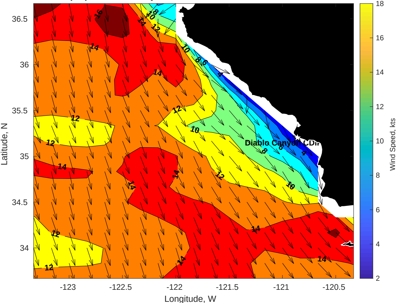
GFS Winds (kts) for Diablo Canyon CDIP GFS at 30-Nov-2025 09:00:00
