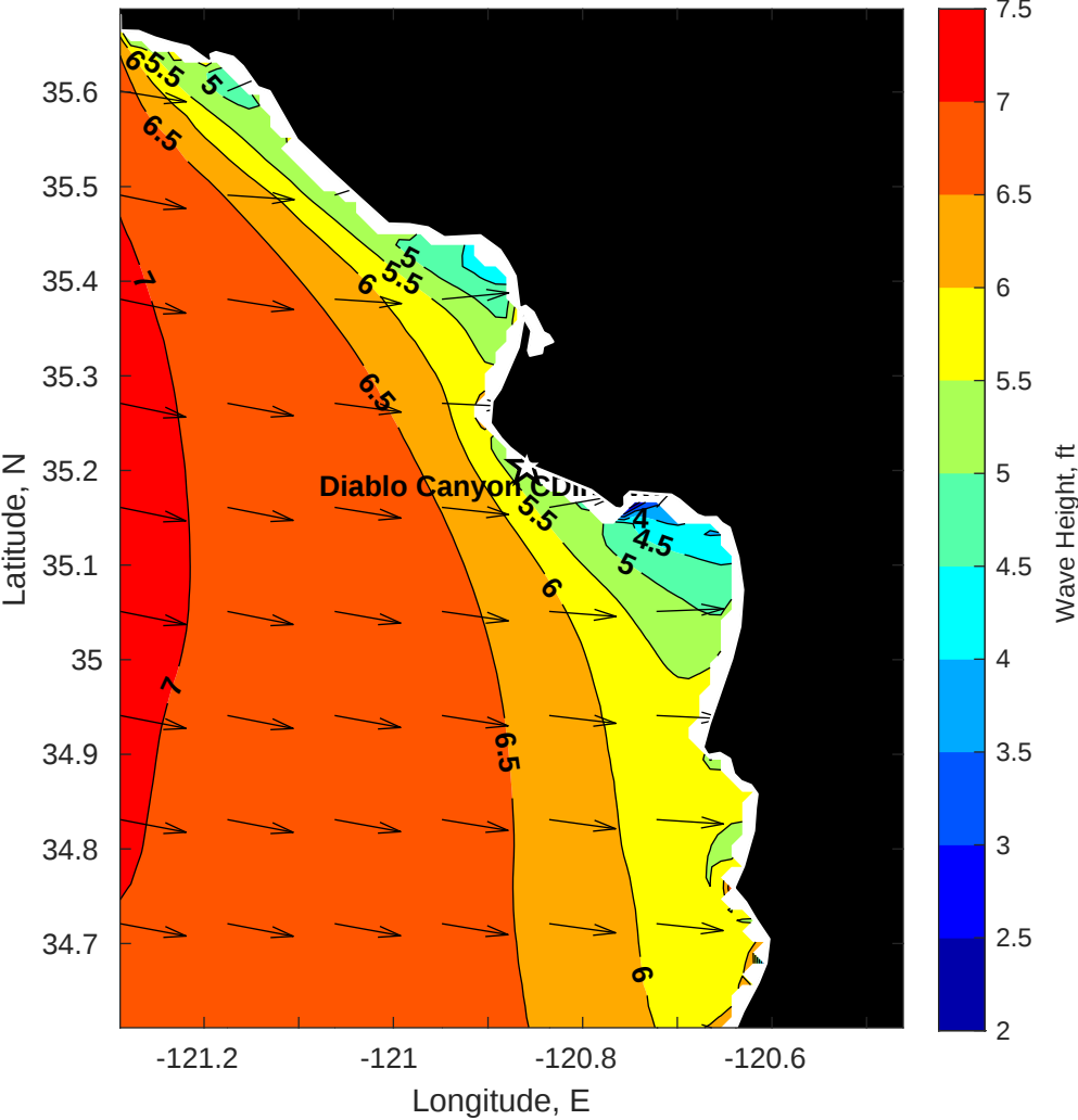
SWAN Wave Height (ft) for Diablo Canyon CDIP SWAN at 30-Nov-2025 10:00:00
