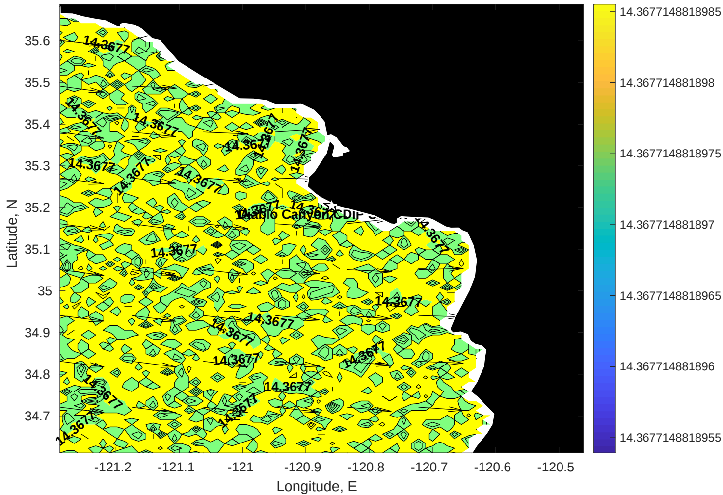
SWAN Wave Period (sec) for Diablo Canyon CDIP SWAN at 30-Nov-2025 10:00:00
