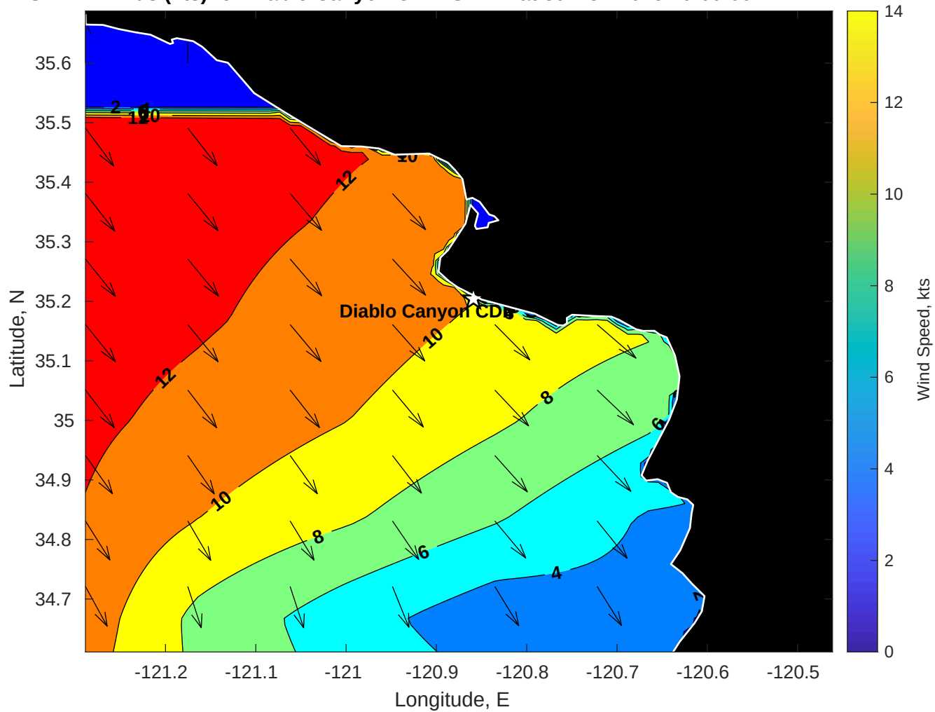
SWAN Winds (kts) for Diablo Canyon CDIP SWAN at 30-Nov-2025 10:00:00
