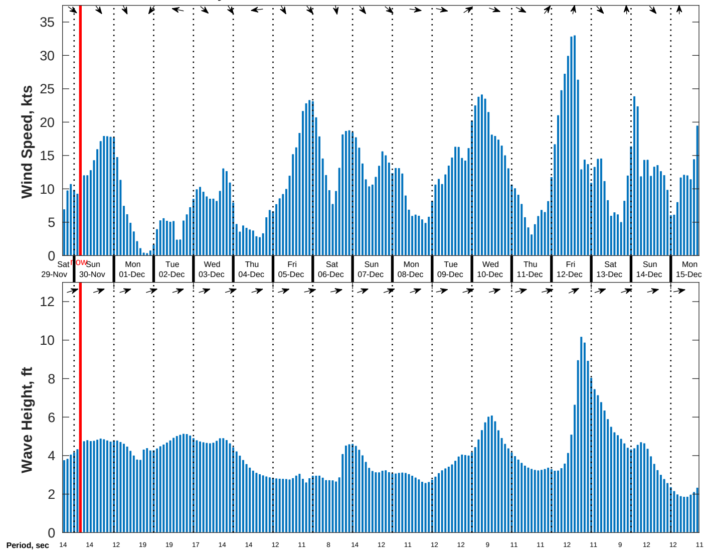
Wind & Wave Forecast for Diablo Canyon CDIP SWAN from 29-Nov-2025 17:00:00 to 15-Dec-2025 17:00:00
