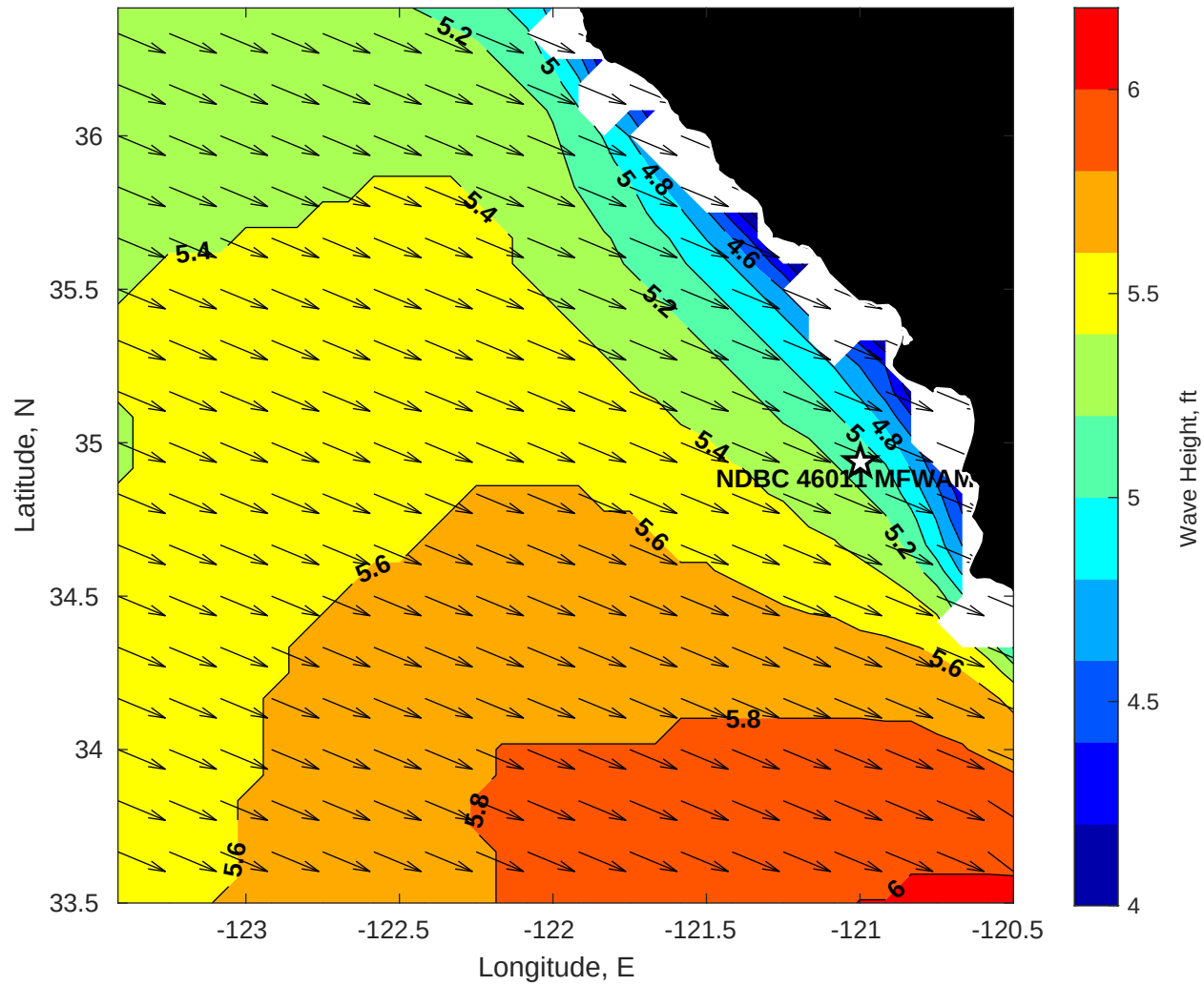
WAM Wave Height (ft) for NDBC 46011 MFWAM at 30-Nov-2025 09:00:00
