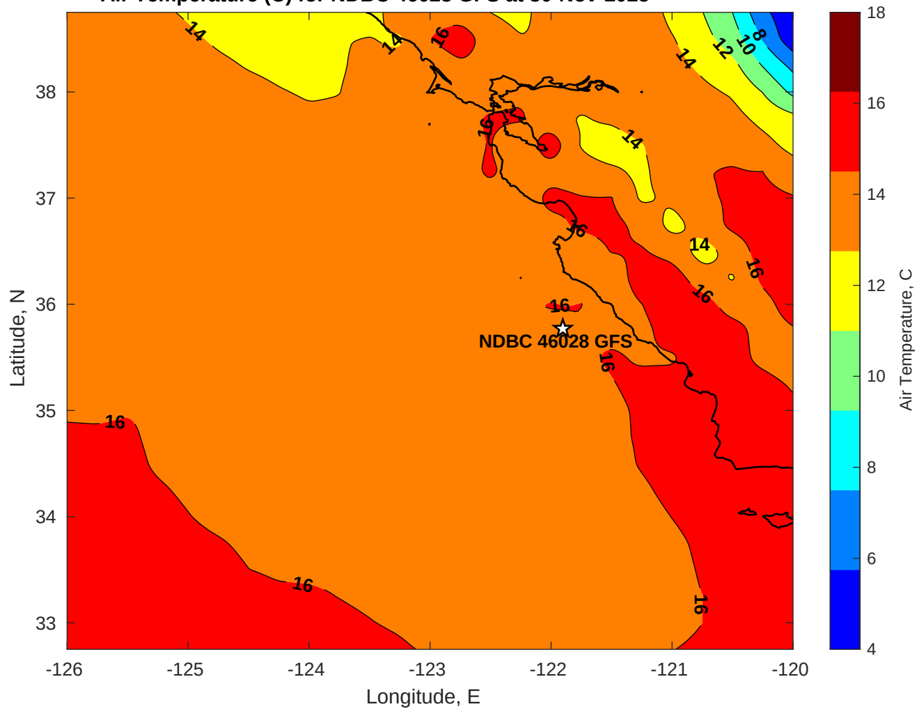
Air Temperature (C) for NDBC 46028 GFS at 30-Nov-2025
