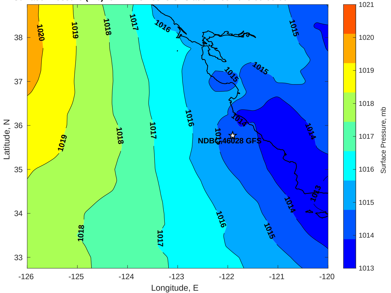
Surface Pressure (mb) for NDBC 46028 GFS at 01-Dec-2025 00:00:00
