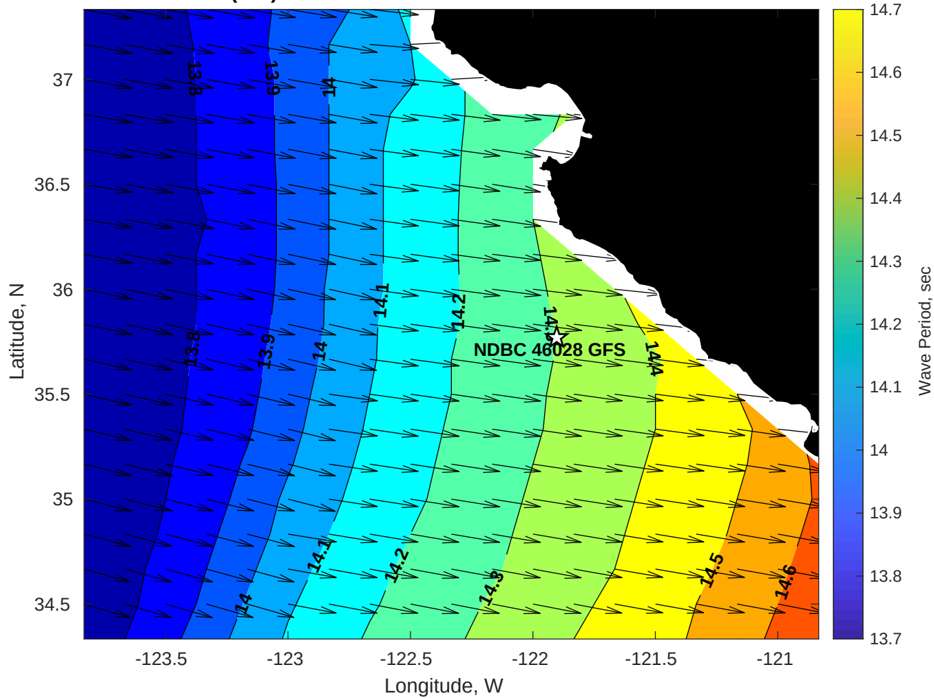
GFS Wave Period (sec) for NDBC 46028 GFS at 30-Nov-2025 09:00:00
