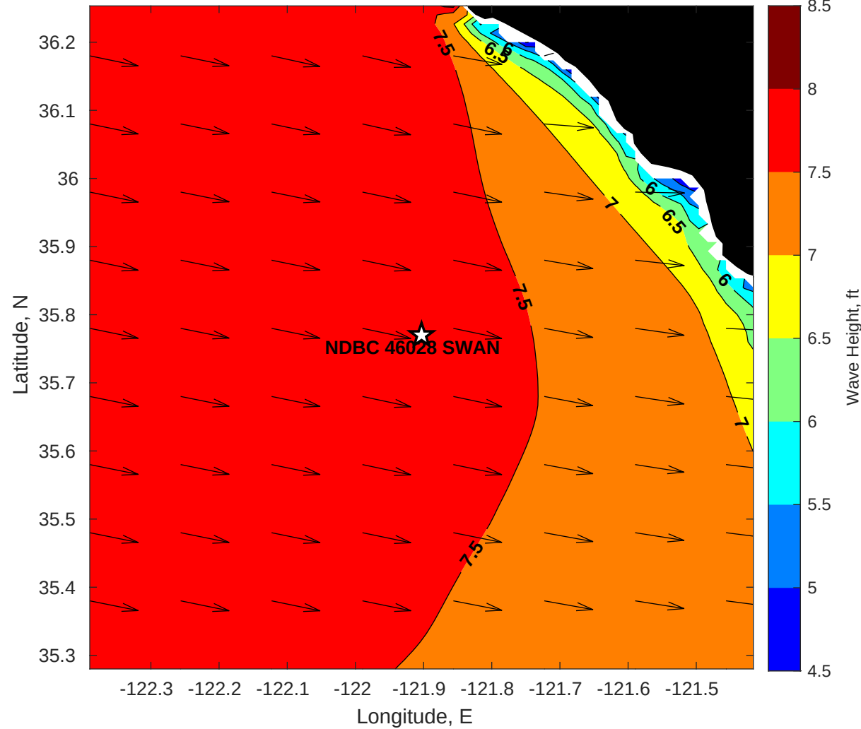
SWAN Wave Height (ft) for NDBC 46028 SWAN at 30-Nov-2025 10:00:00
