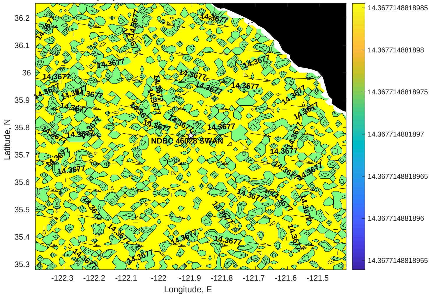
SWAN Wave Period (sec) for NDBC 46028 SWAN at 30-Nov-2025 10:00:00
