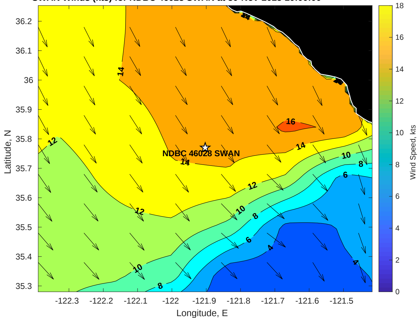
SWAN Winds (kts) for NDBC 46028 SWAN at 30-Nov-2025 10:00:00
