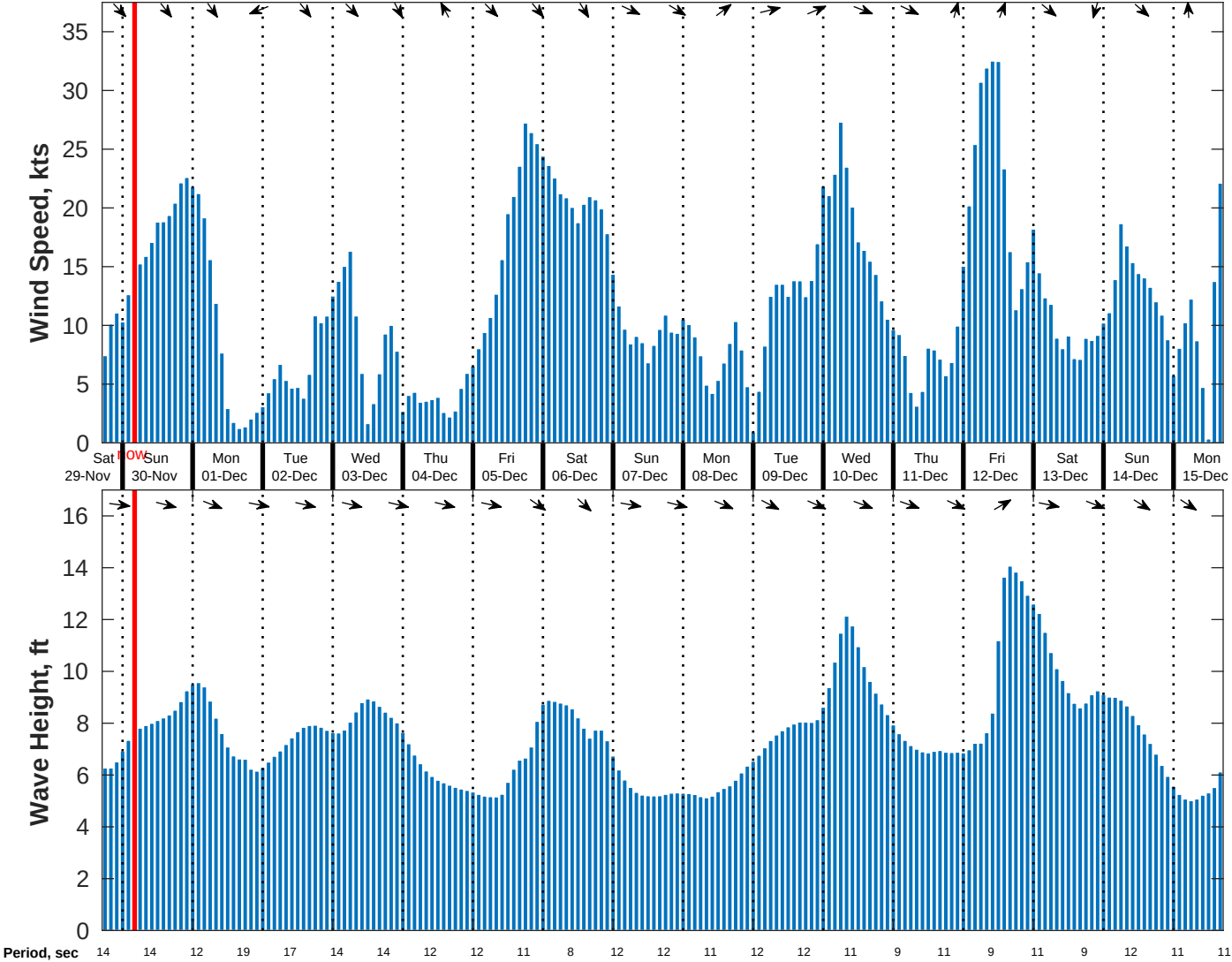
Wind & Wave Forecast for NDBC 46028 SWAN from 29-Nov-2025 17:00:00 to 15-Dec-2025 17:00:00
