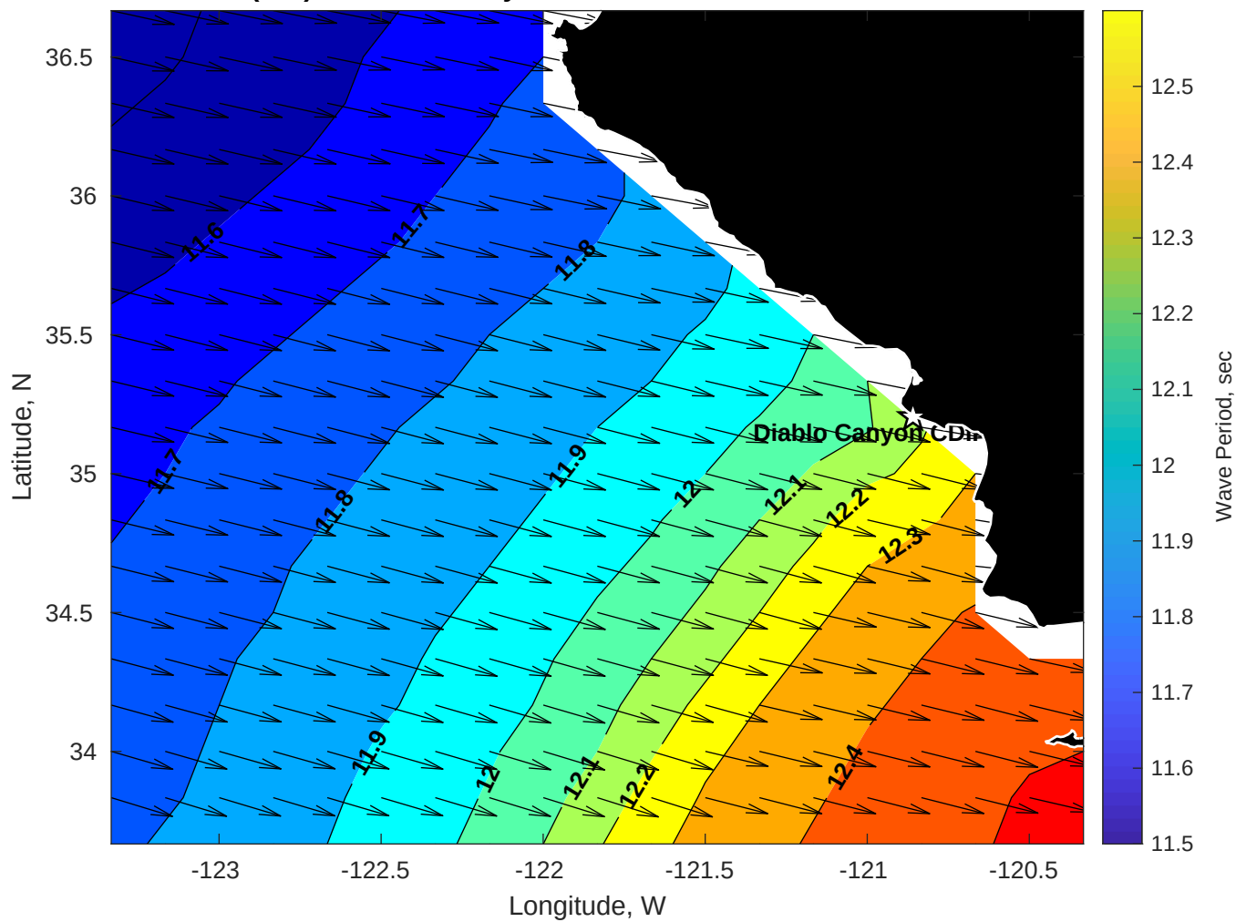
GFS Wave Period (sec) for Diablo Canyon CDIP GFS at 01-Dec-2025 09:00:00
