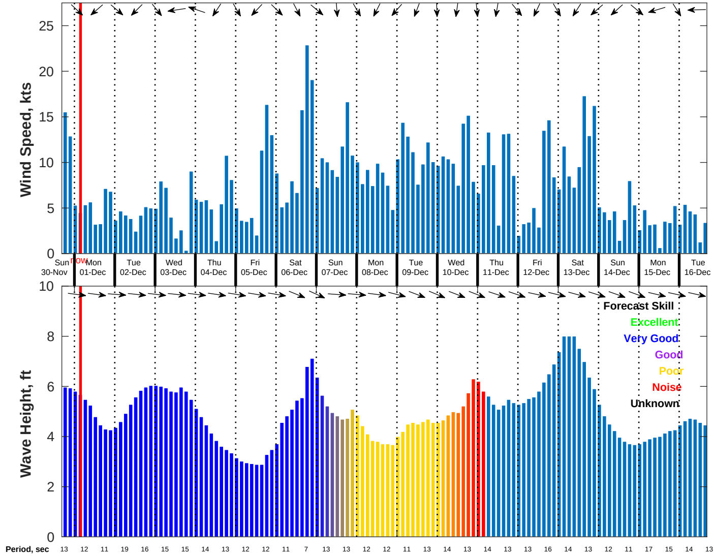
Wind & Wave Forecast for Diablo Canyon CDIP GFS from 30-Nov-2025 17:00:00 to 16-Dec-2025 17:00:00
