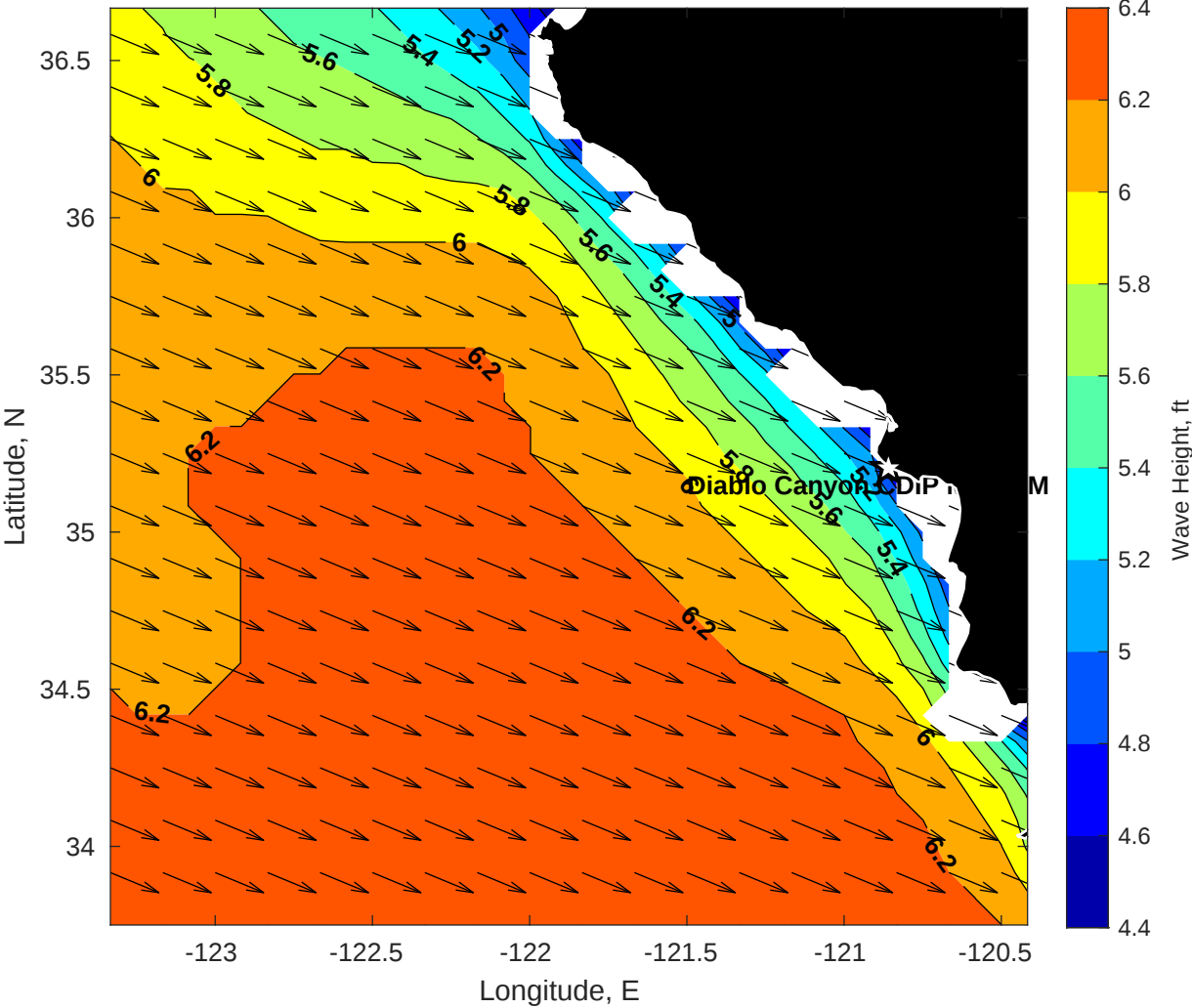
WAM Wave Height (ft) for Diablo Canyon CDIP MFWAM at 01-Dec-2025 09:00:00
