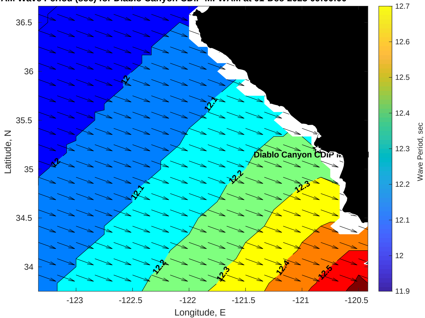
WAM Wave Period (sec) for Diablo Canyon CDIP MFWAM at 01-Dec-2025 09:00:00
