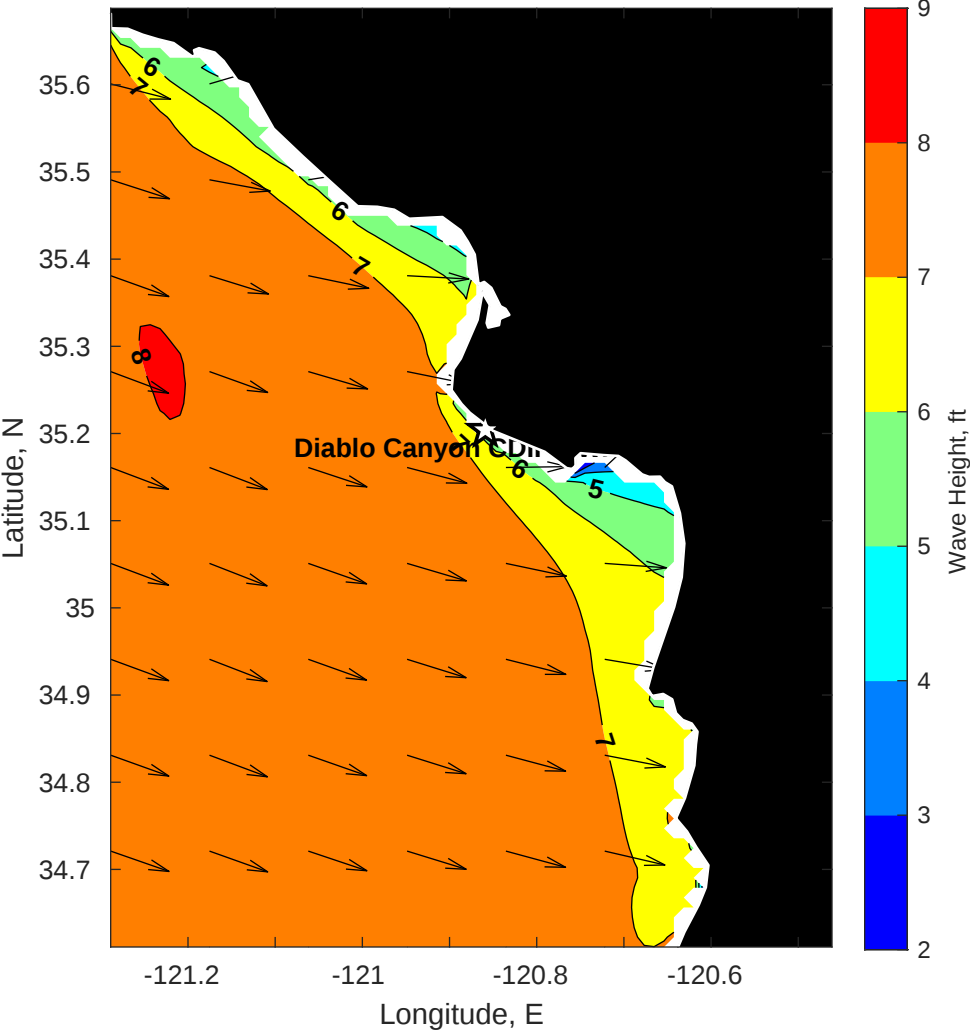
SWAN Wave Height (ft) for Diablo Canyon CDIP SWAN at 01-Dec-2025 10:00:00
