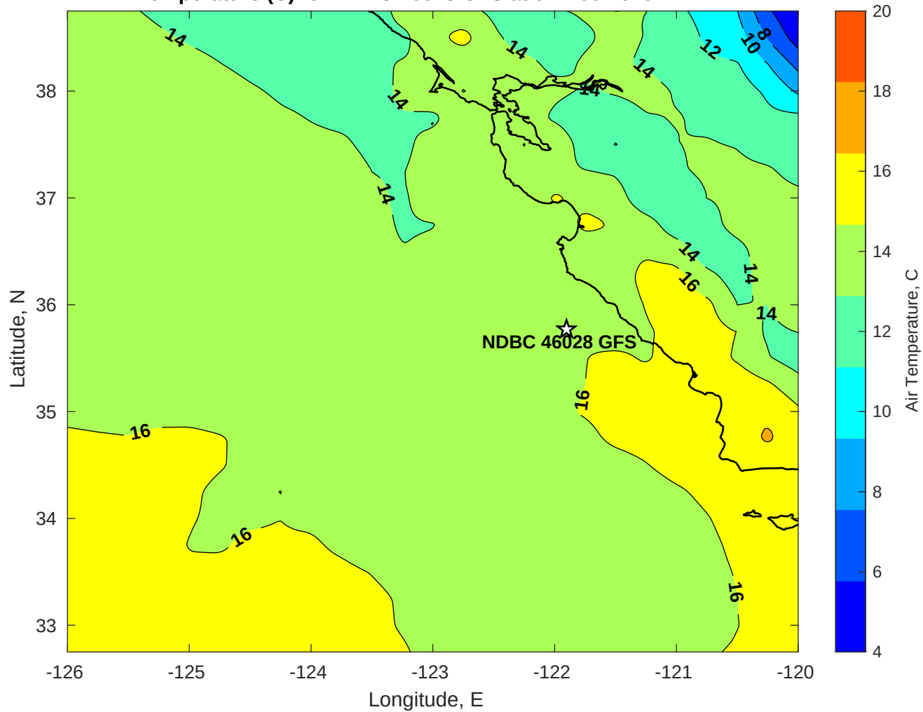
Air Temperature (C) for NDBC 46028 GFS at 01-Dec-2025
