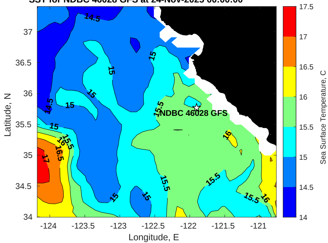
SST for NDBC 46028 GFS at 24-Nov-2025 00:00:00
