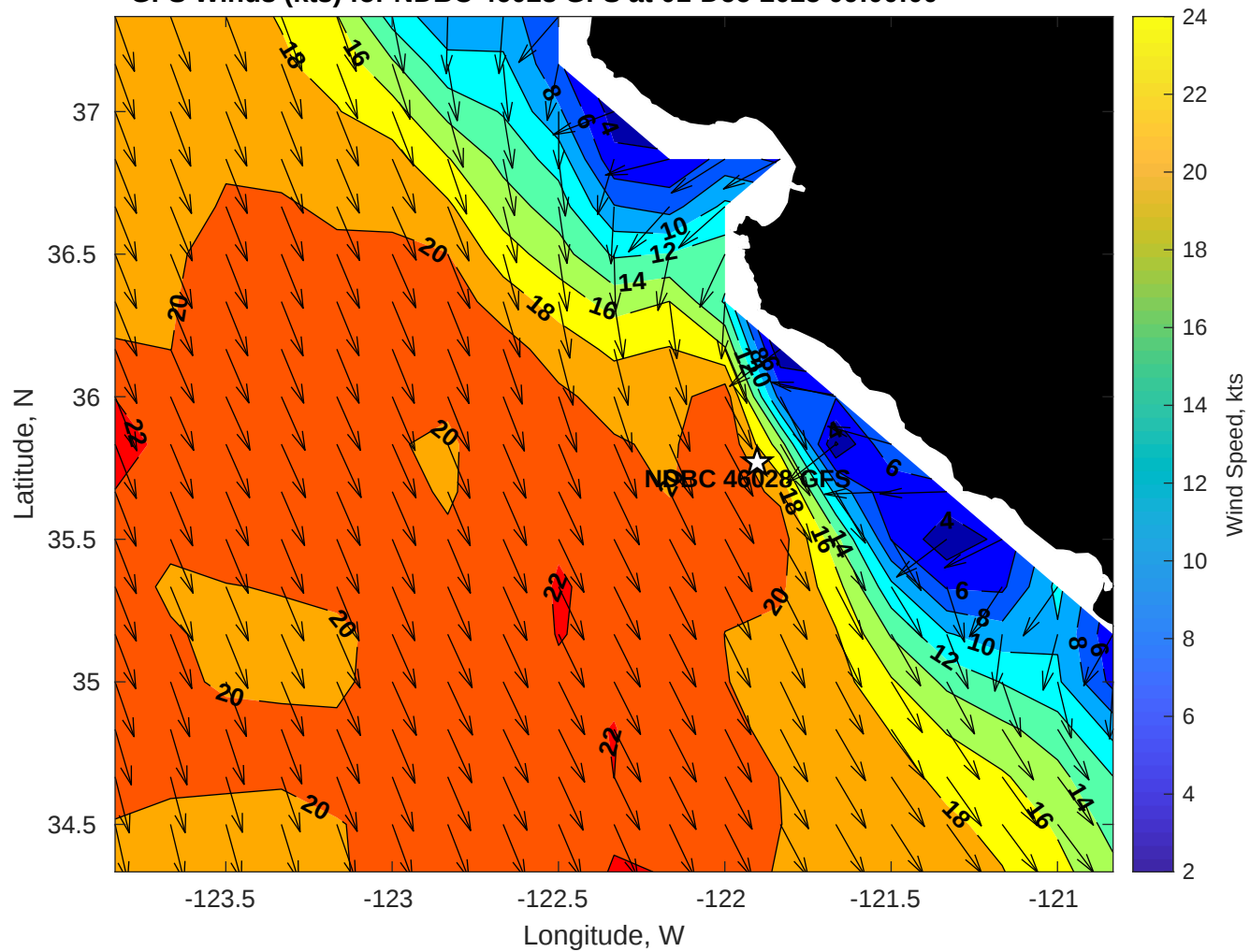
GFS Winds (kts) for NDBC 46028 GFS at 01-Dec-2025 09:00:00
