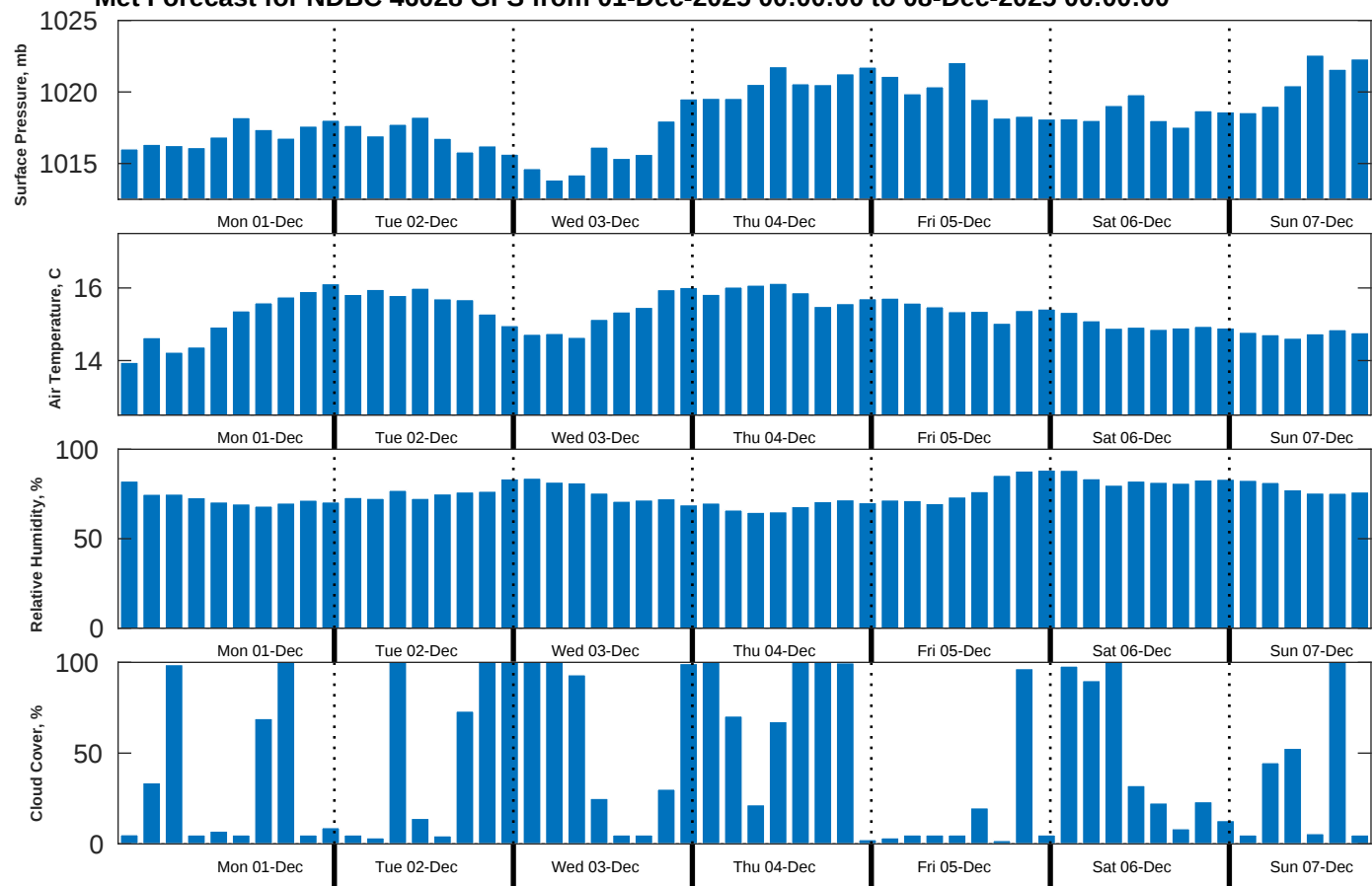
Met Forecast for NDBC 46028 GFS from 01-Dec-2025 00:00:00 to 08-Dec-2025 00:00:00
