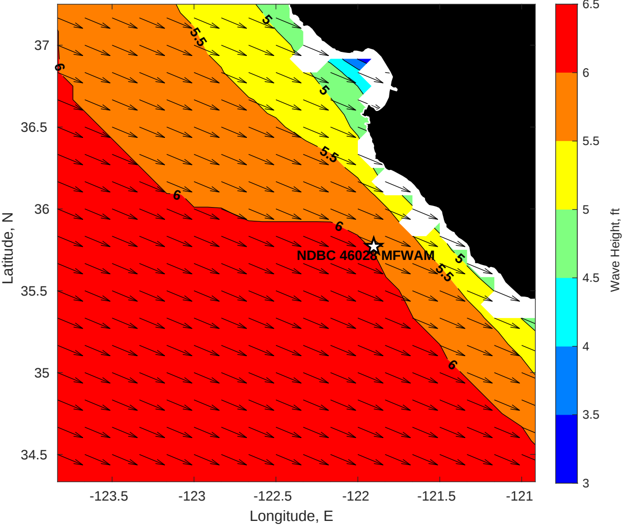
WAM Wave Height (ft) for NDBC 46028 MFWAM at 01-Dec-2025 09:00:00
